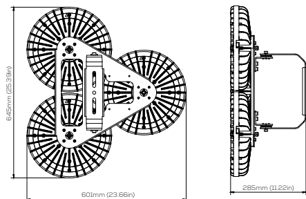
3 modules (450W)
